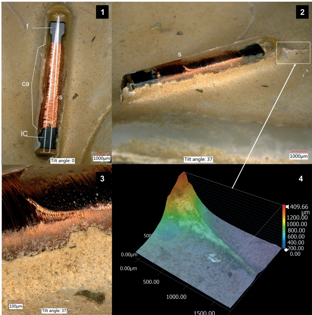
Figs 1–4. PIT tag attached to the shell of U. crassus , found empty in 2015, in the sediment of the bank of the San River: 1 – relative arrangement of the basic elements (ca – coil antenna, f – ferrite core, IC – integrated circuit, s – silicone layer edge), 2 – PIT tag incorporated in the inner shell layer, 3 – close-up view of the thickness and structure of nacre layer, partially removed from the glass of the transponder, 4 – dimensions of the buttress built at the PIT tag end in relation to the elevation
