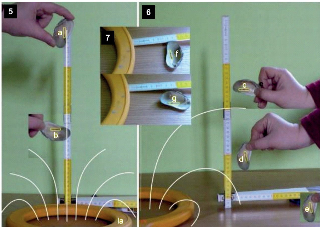
Figs 5–7. Activating distances of the PIT tag in relation to the distance to the large inducing antenna and the lines of its electromagnetic field (white lines): 5 – activation of PIT tag in the centre of inducing coil antenna (a – PIT tag oriented along the main lines of electromagnetic field, b – PIT tag oriented perpendicularly to the lines – the distance of activation decreases significantly, la – loop antenna), 6 – activation of PIT tag outside the inducing coil antenna (c – despite the horizontal position of the tag, outside the large coil, it conforms to the lines and is activated at a significant distance, d – position of the tag changed, but because the tag orientation conforms to the lines the distance of activation remains large, e – at the plane of the loop the effective position of the tag is vertical, conforming to the field lines), 7 – activation of the tag in the horizontal plane of the inducing antenna (f, g – horizontal positions of both the PIT tags do not conform to the lines which are vertical, thus the distance of activation is significantly reduced in comparison to (e))
